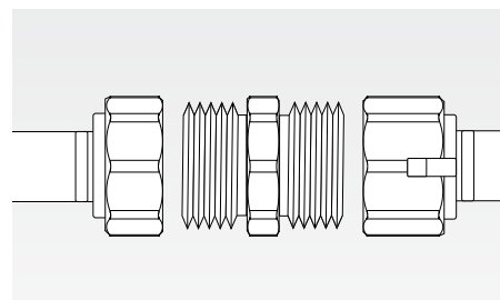
Straight pipe connector break-down
