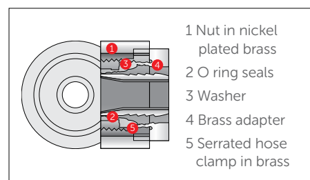
Straight pipe connector break-down
